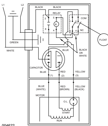
WIRING DIAGRAM FOR MODELS "D284-B", "D284-C", and "D284-D" 9/86 (VS) thru Current
