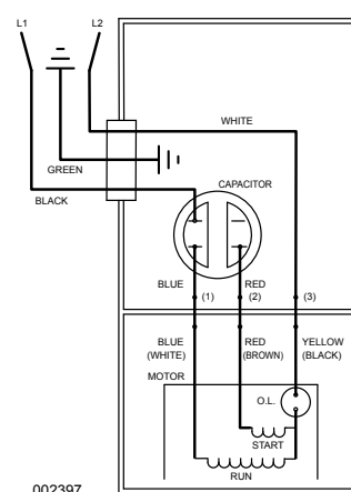
WIRING DIAGRAM FOR MODELS "E284-A", "E284-B", "E284-C", and "E284-D" 11/81 (XM) thru Current
