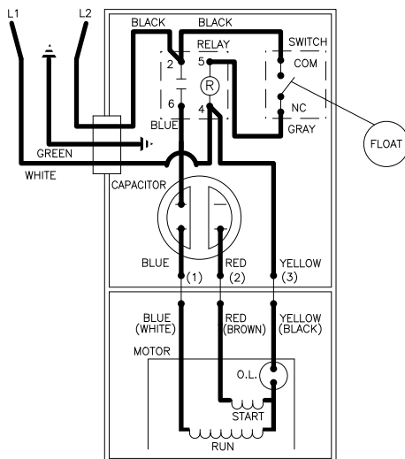
WIRING DIAGRAM FOR MODELS "D293-A" 12/80 (YJ) thru 8/96 (US)
