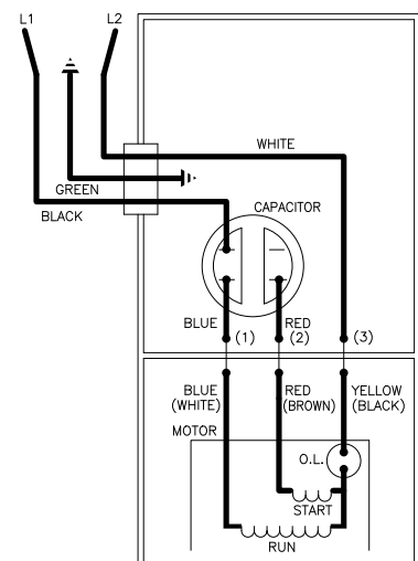
WIRING DIAGRAM FOR MODELS "E293-A", "E293-B", "E293-C", & "E293-D" 12/80 (YJ) thru Current
