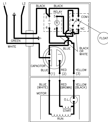
WIRING DIAGRAM FOR MODELS "D293-B", "D293-C", & "D293-D" 9/86 (VS) thru Current
