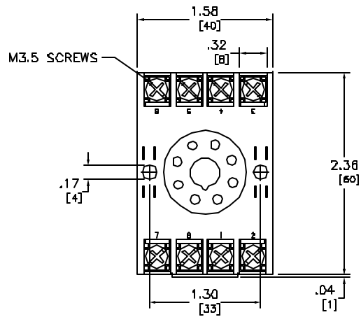
FRONT VIEW SHOWN WITHOUT RELAY INSTALLED
