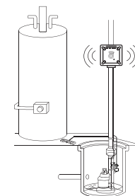
Sump Pump with High Level and Overflow/Utility Room Leak Detection
