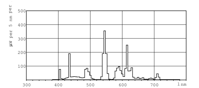
LDPB_TL5-HE8_835-Spectral power distribution B/W
