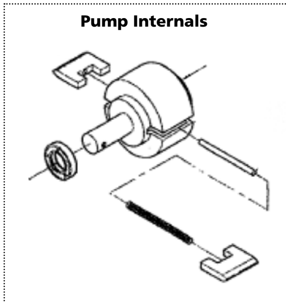
Figure 4- Repair Parts Illustration for Dayton® Rotary Barrel Pump
