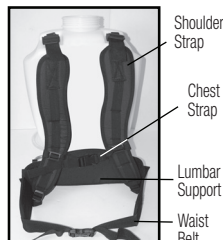
Figure 1 Strap Assembly
