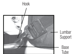
Figure 2 Hook Attachment
