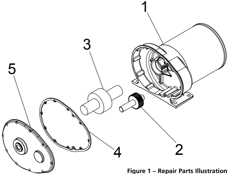
Figure 1 – Repair Parts Illustration 1LPU3, 1LPU4 and 1LPU5
