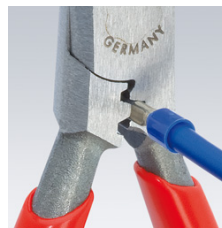
Crimping 0.5 to 2.5 mm 2 / AWG 14 - AWG 20
